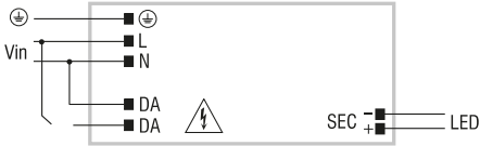
PUSH SWITCH diagram Collegamento PUSH SWITCH
