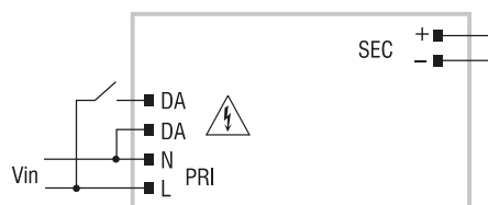
PUSH SWITCH diagram Collegamento PUSH SWITCH
